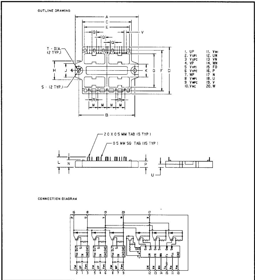
110-230 Volt Line, PM20CEA060 Outline Drawing
